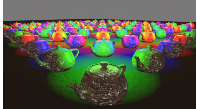
Figure 8: A scene with 101 objects and 81 omni lights running at 34fps (29.4ms) with inferred lighting on the Xbox 360. This same scene runs at 6fps (167ms) with forward rendering.
